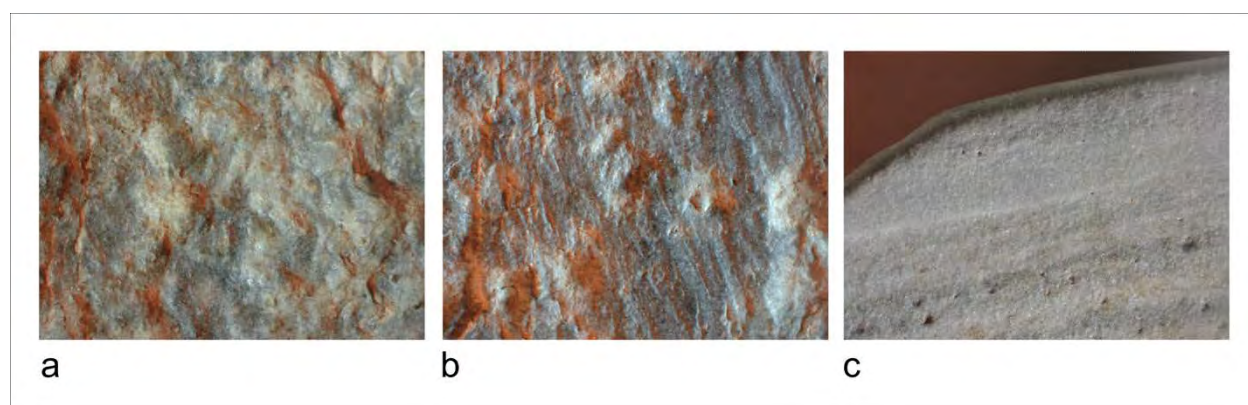
Figure 13. Microscopic images of fragmented celt surfaces
